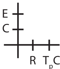
FIGURE 4. Image of the Pointed Brill-Noether Divisor BN_{6,(0,2,4)}^2
