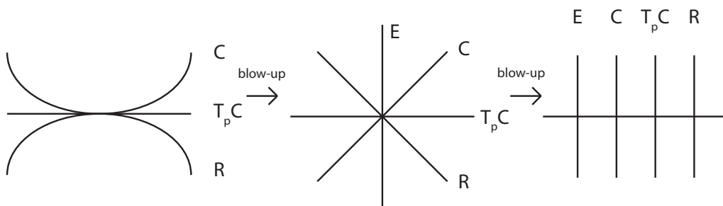
FIGURE 1. The map \phi_5
