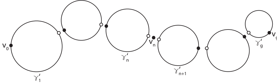
FIGURE 2. Cell decomposition of the graph \Gamma_g (from [CDPR])
