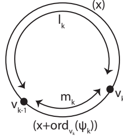
FIGURE 3. The slopes of \psi (outside the loop) and distances (inside the loop) on \tilde{\gamma}_k
