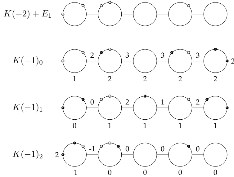
FIGURE 6. Divisors in the linear system K_\Gamma - g_3^1 .
