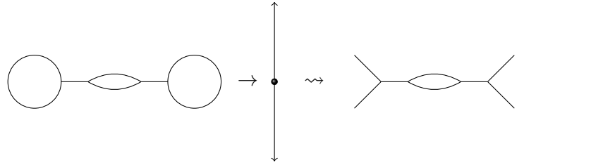
FIGURE 10. The figure on the left shows a superabundant tropical curve. The map is given by projection onto the vertical axis. The center cycle has been made thin to indicate that it is contracted. The figure on the right shows a neighborhood of 0 in the target and a connected component of its preimage. We suppress the trees attached to the cycles for clarity.
