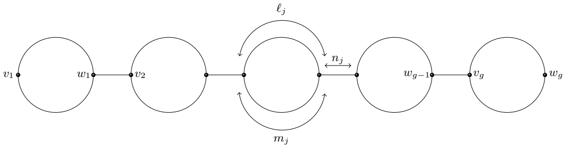
FIGURE 2. The chain of cycles \Gamma .
