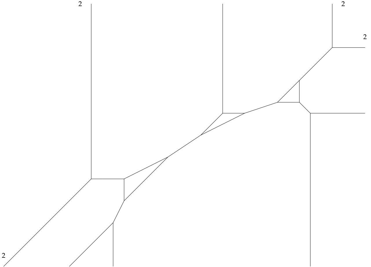
FIGURE 7. The image of \Gamma in \mathbb{F}_1^{\text{trop}} . The map is manifestly superabundant, since the image has genus 3 and \Gamma is a chain of 5 cycles.
