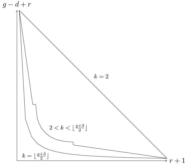
FIGURE 1. This graph shows the points (r + 1, g - d + r) for which W_d^r(C) is nonempty, when C is a general curve of gonality k , for various values of k .
