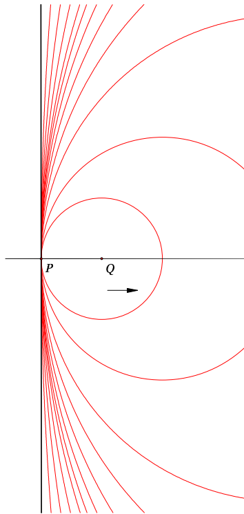
Figure 11.1: Circles converging to a perpendicular line in the Euclidean plane
