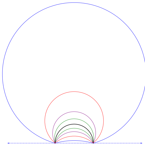
Figure 11.3: Concentric hypercycles in the Poincaré Half Plane model
