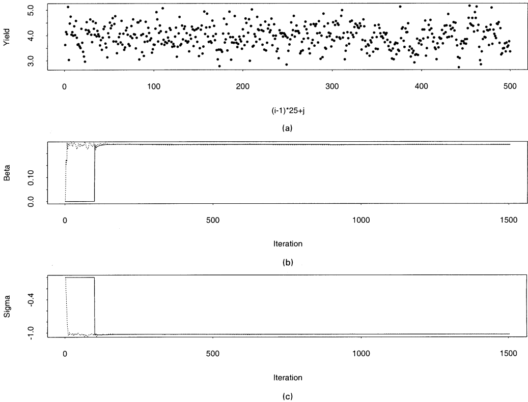
Fig. 2. Mercer and Hall's wheat yield data: (a) yields against (i - 1) \times 25 + j , where (i, j) denotes a site on a 20 \times 25 rectangular lattice; (b) \beta^k (.....) and \hat{\beta}^k (——) at each iteration of the Markov chain Monte Carlo stochastic approximation algorithm; (c) \sigma^{*k} (.....) and \hat{\sigma}^{*k} (——) at each iteration of the Markov chain Monte Carlo stochastic approximation algorithm
