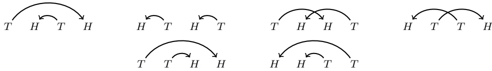
Figure 7: The rules for pairs of arrows in the Simion type c subclass.
