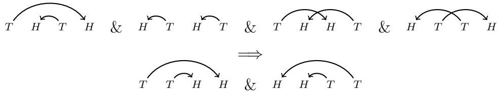
Figure 2: A graphical representation of Proposition 3.7.
