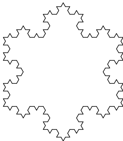
4th stage of the snowflake curve
