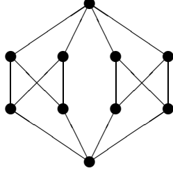
Figure 2: A finite Sheffer poset with the same factorial functions as the cubical lattice.
