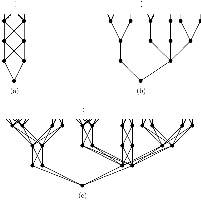
Figure 1: (a) the infinite butterfly poset \mathbb{T} , (b) an infinite tree Q , (c) and the rank product \mathbb{T} * Q , which has the same factorial function as the butterfly poset.
