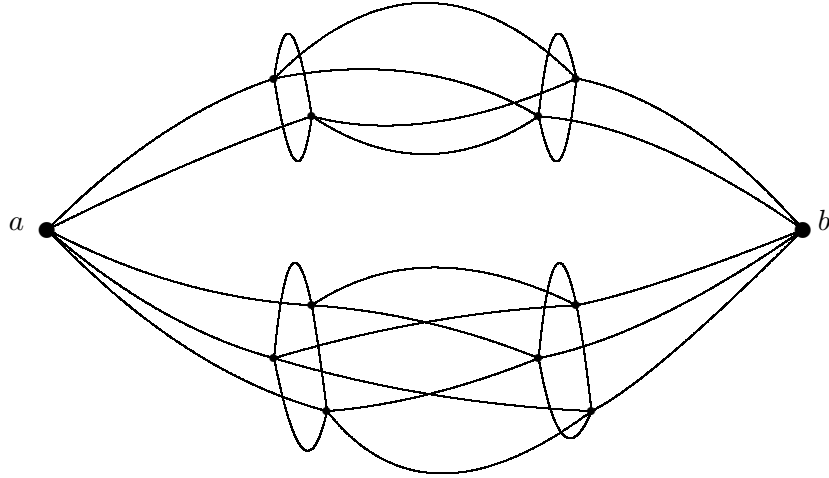
Figure 3: The CW-complex obtained by joining the complexes X_2 and X_3 at the vertices a and b .
