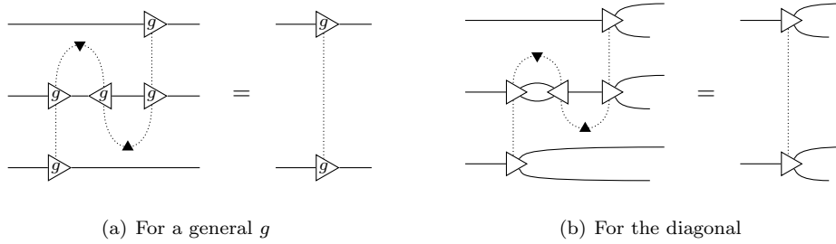
FIGURE 15. Triangle identities for the adjunctions g_! \dashv g^*
