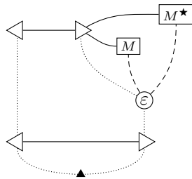
(e) The bicategorical evaluation in terms of the symmetric monoidal one
