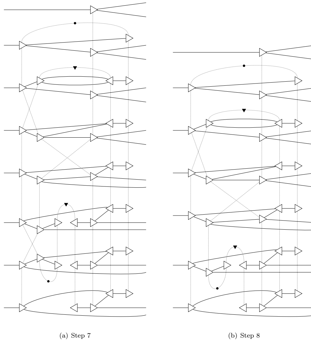
FIGURE 30. Upper part IV, from the proof of Theorem 6.9(i)
