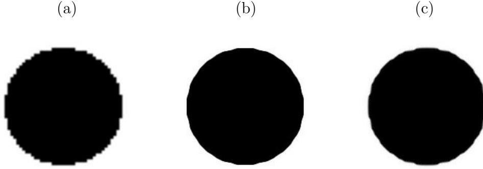
Figure 4: Synthetic binary images in 240 \times 240 cells, for magnification of 4 \times 4 . (a) The interpolated image by H_2^{\text{cubic}} from an image in 60 \times 60 cells, (b) the edge-formed image by \mathcal{D}_1 (3.16), and (c) the edge-formed image by \mathcal{D}_2 (3.17).
