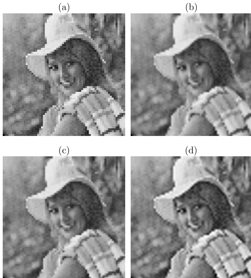
Figure 1: The Elaine image in 256 \times 256 cells interpolated from a small image of 64 \times 64 pixels, by (a) H_1 , (b) H_2 , (c) H_2^{\text{cubic}} = H_{4,0} , and (d) H_{4,-3/4} .
