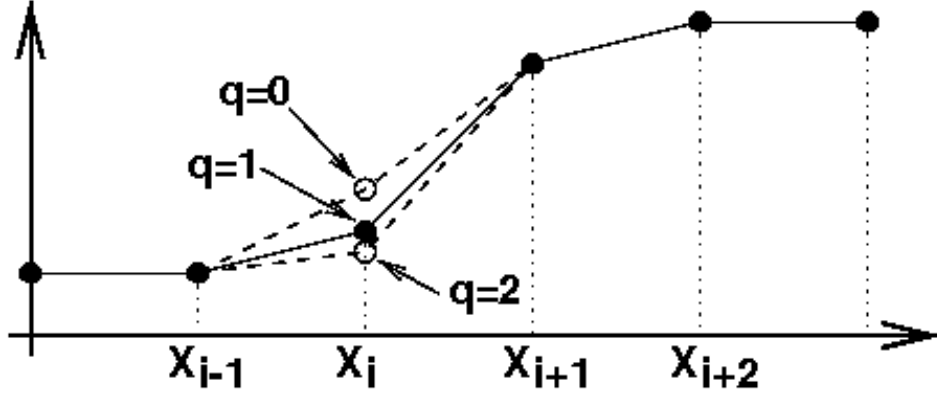
Figure 2: The edge-forming principle. The solid curve involving solid circles is the solution at the previous level u^{n-1} and the dashed curves indicate the solutions in the current level near the point x_i depending on q .
