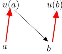
Figure 2.3: First three steps of a gradient path.
