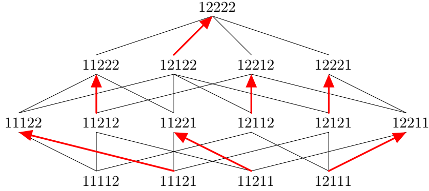
Figure 1: The matching of the Stirling poset \Pi(5, 2) .
