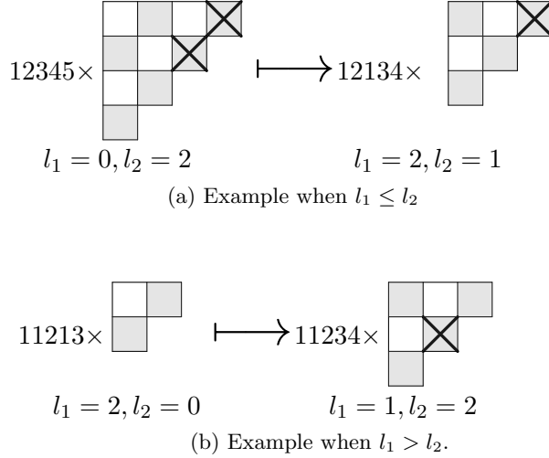
Figure 10: Examples of the bijection proving the identity (9.10).
