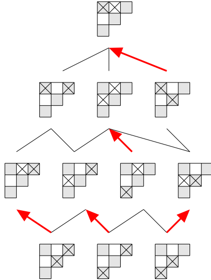
Figure 7: Example of \Gamma(4, 2) with its matching. There is one unmatched rook placement in rank 2.
