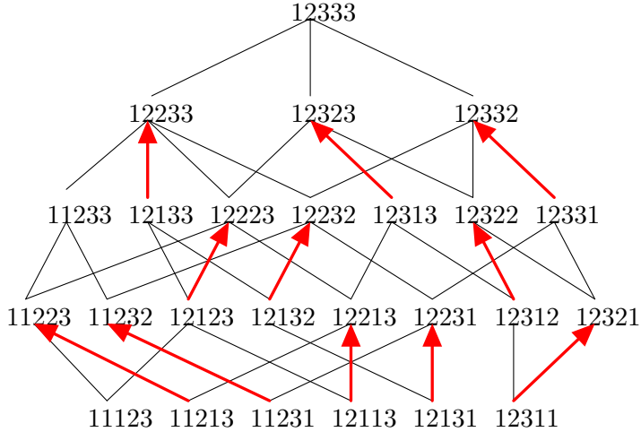
Figure 2: The Stirling poset \Pi(5, 3) and its discrete Morse matching. The rank generating function is the q -Stirling number S_q[5, 3] = q^4 + 3q^3 + 7q^2 + 8q + 6 . The matched elements are indicated by arrows. The unmatched elements are 11123, 11233 and 12333, and the sum of their weights is 1 + q^2 + q^4 .
