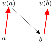
Figure 3: First three steps of a gradient path.
