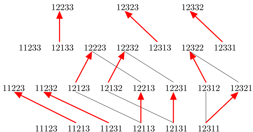
Figure 5: The decomposition of the Stirling poset \Pi(5, 3) into Boolean algebras. Again, the matched elements are indicated with arrows. The weight of the poset is S_q[5, 3] = 1 + 2(1 + q) + 3(1 + q)^2 + q^2 + 3q^2(1 + q) + q^4 .
