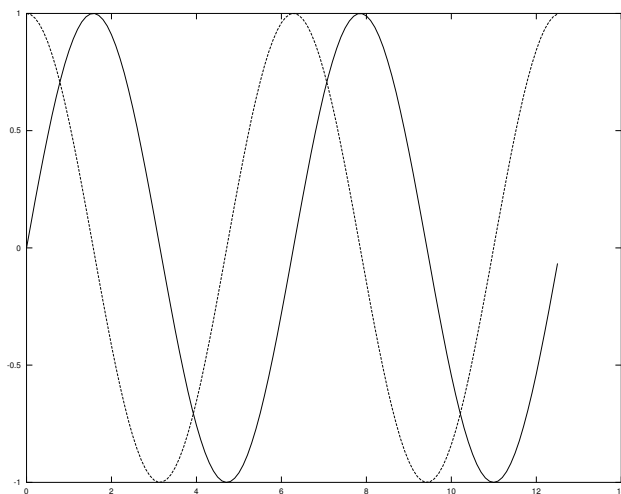
Figure 1: The graph of \sin(x) and \cos(x)
