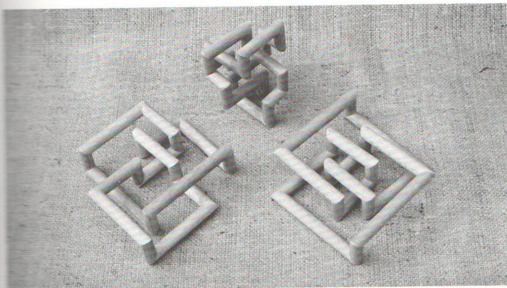
Figure 3.5 Topologically these three versions of Listing's Knot are all alike: each has four irreducible crossings.
