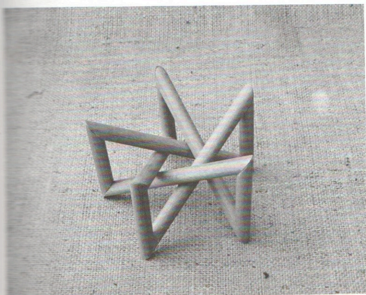
Figure 3.6 The cinquefoil knot is an especially handsome Gordian knot.
